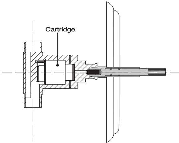
Cutaway View
