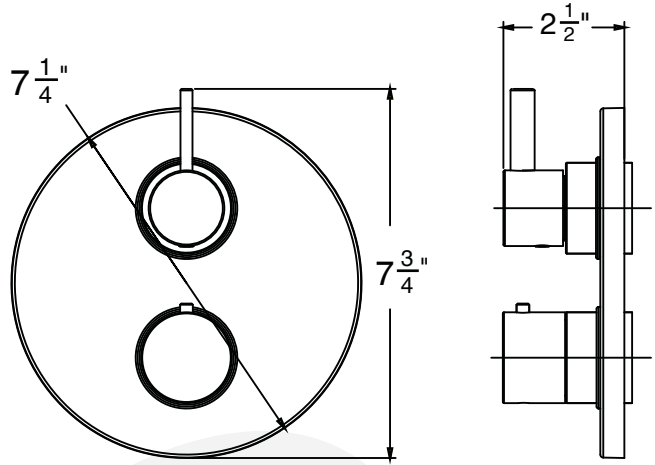
Valve Trim
